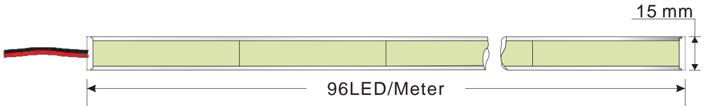
Top View
