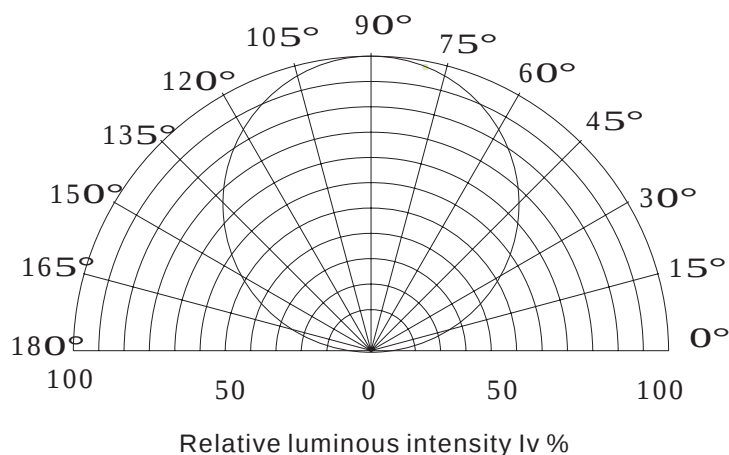
Radiation diagram
